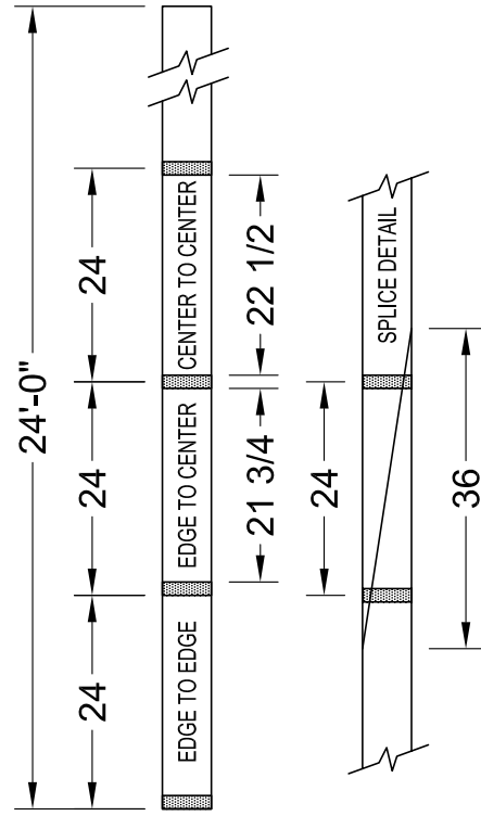
RIDGE LAYOUT
